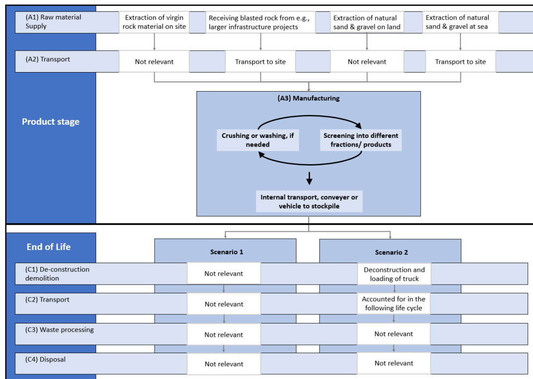
Figure 3: System boundaries for the studied product system.
