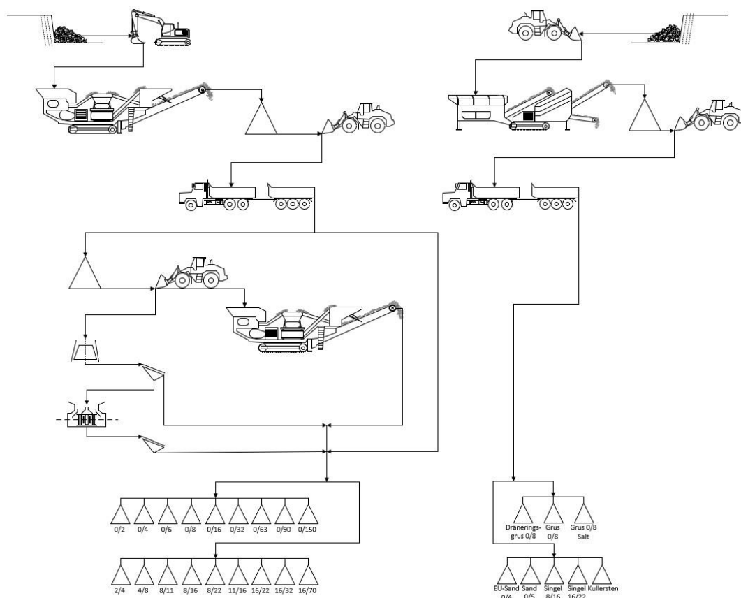
Figure 1: Process set-up for the production of aggregates at the declared site.
