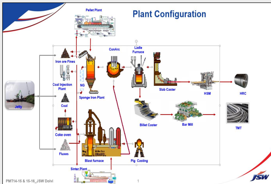
Figure 3 Steel making process at JSW Steel – Dolvi
