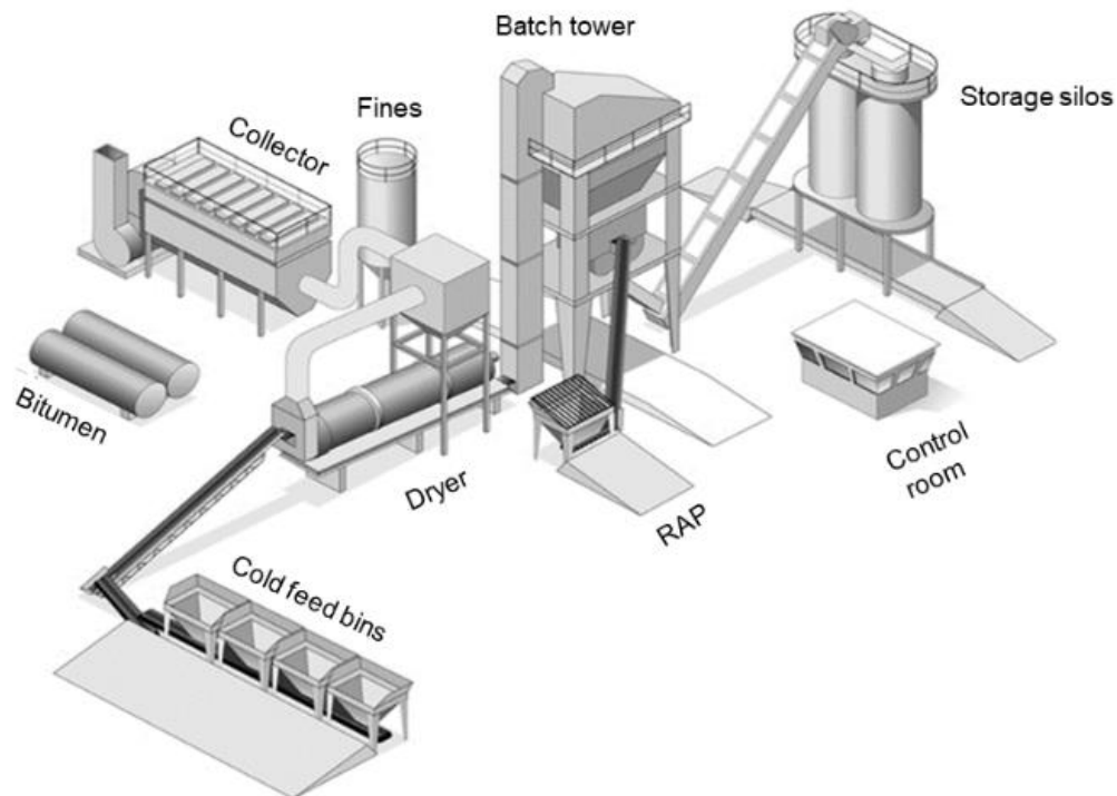
Figure 1: Schematic illustration of an asphalt plant.
