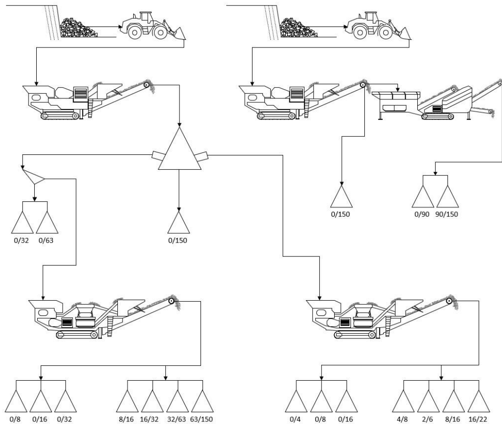
Figure 1: Process set-up for the production of aggregates at the declared site.
