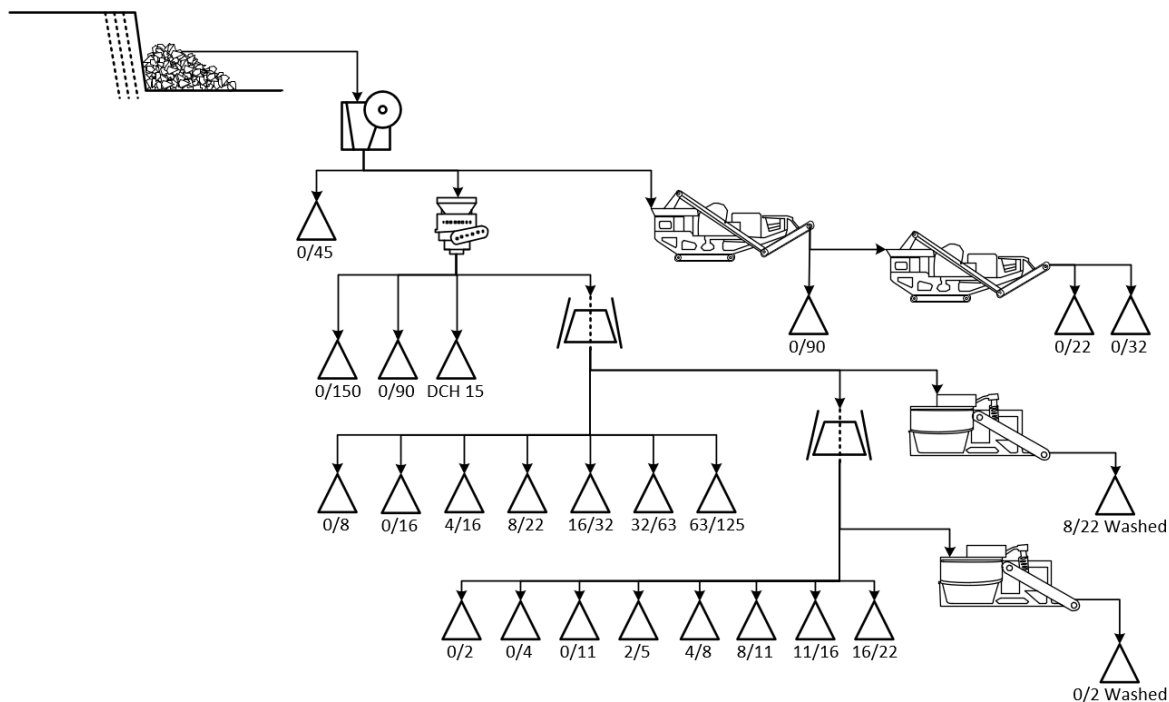
Figure 1: Process set-up for the production of aggregates at the declared site.
