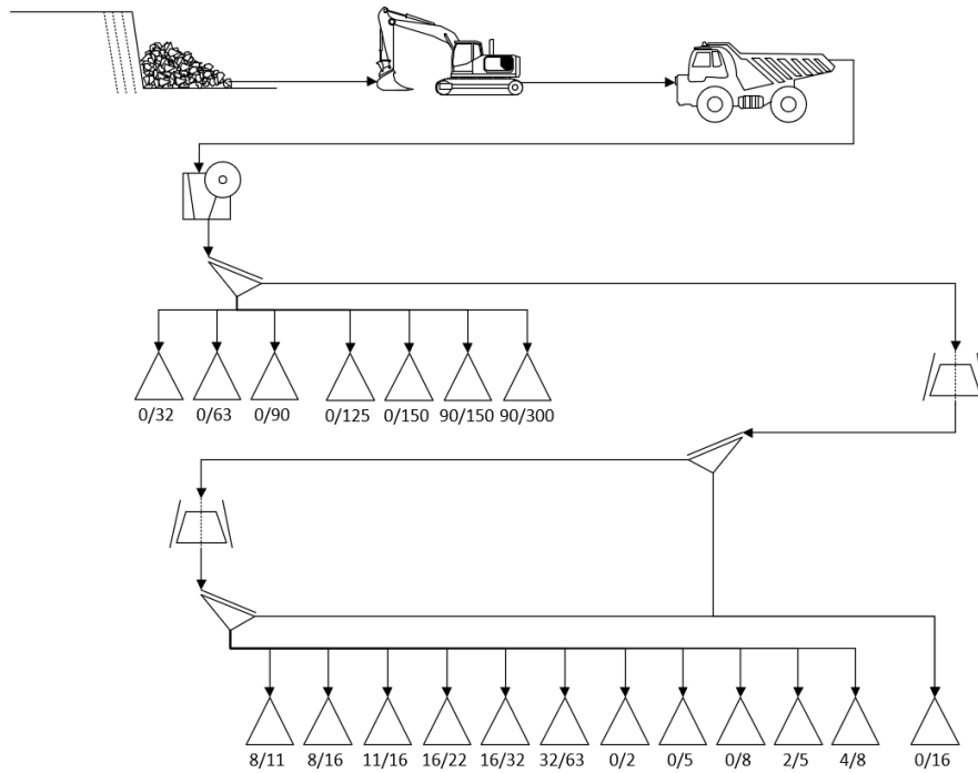
Figure 1: Process set-up for the production of aggregates at the declared site.
