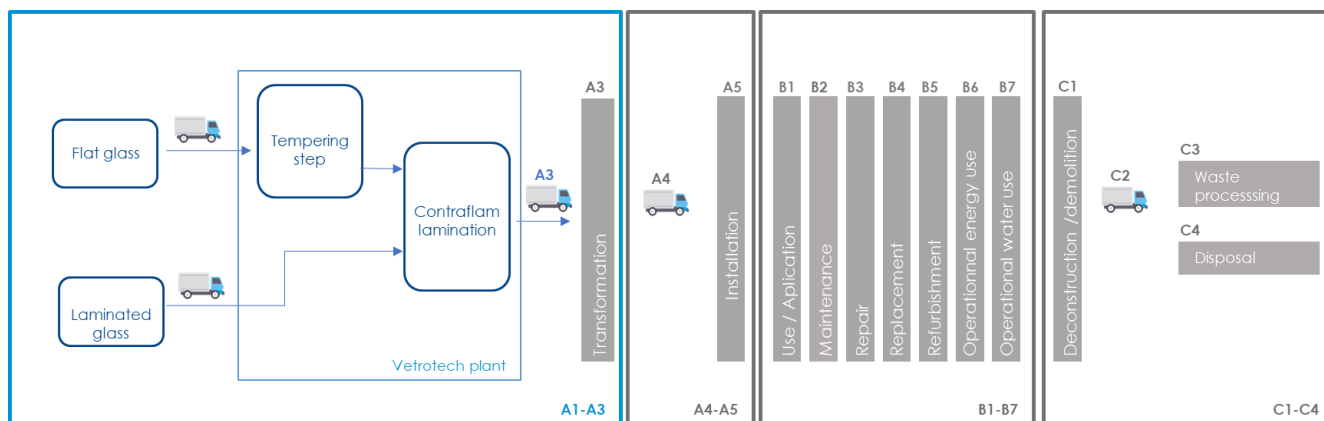
Figure 2 : Relevant LCA steps for Contraflam (44.2/5). Steps in blue are declared in this EPD, steps in grey are not declared.
