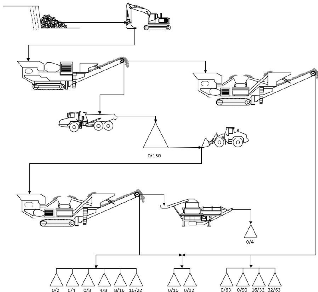
Figure 1: Process set-up for the production of aggregates at the declared site.
