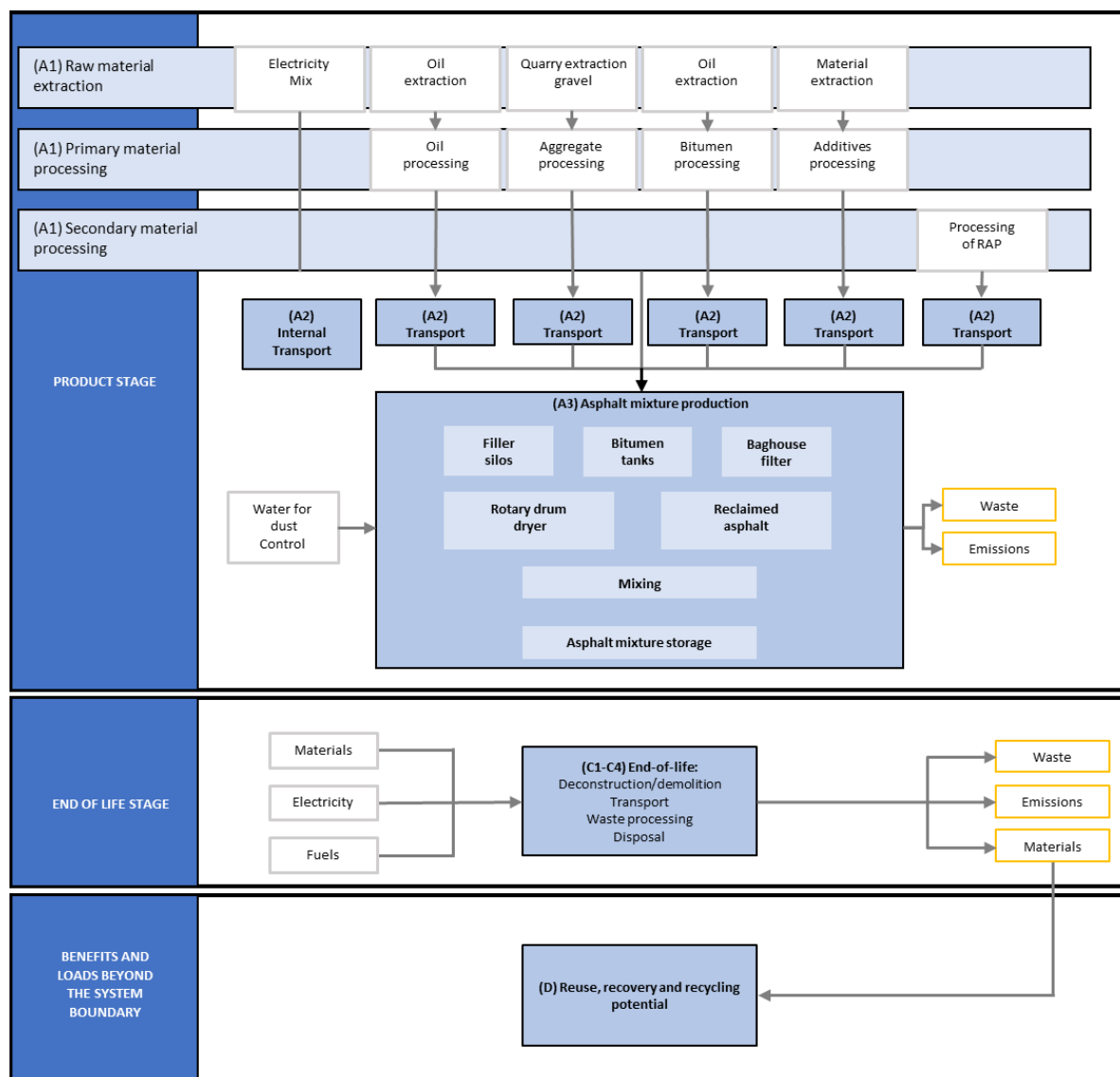
Figure 5: System boundaries for the studied product system.
