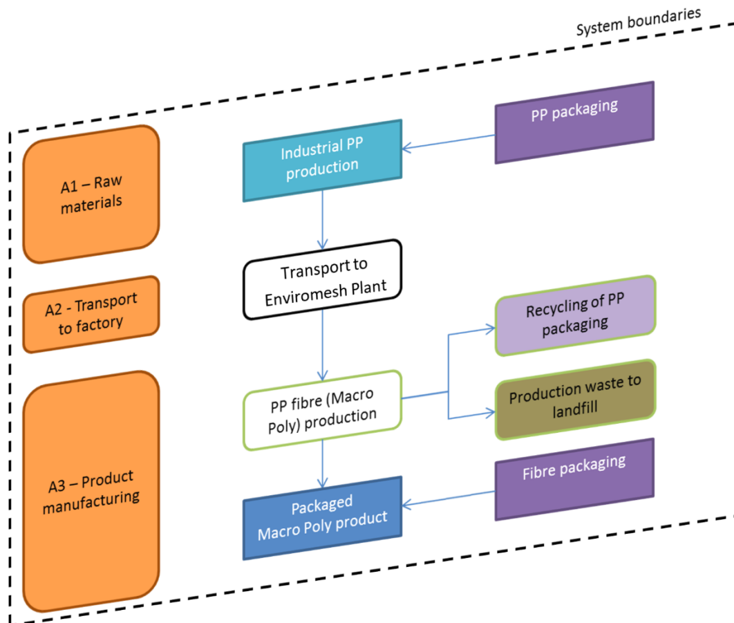
Figure 2. System boundaries for the virgin Macro Synthetic products LCA
